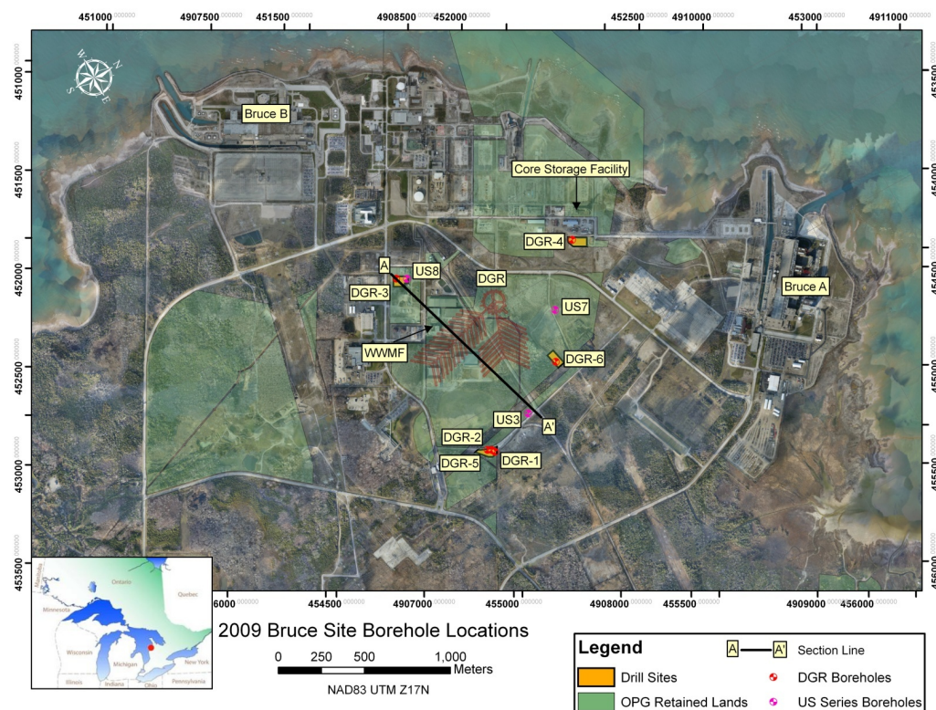
Figure 3: Bruce site base plan showing location of WWMF, proposed DGR layout, DGR Drill sites; DGR(deep)- and US(shallow)-series boreholes and Core Storage Facility.
