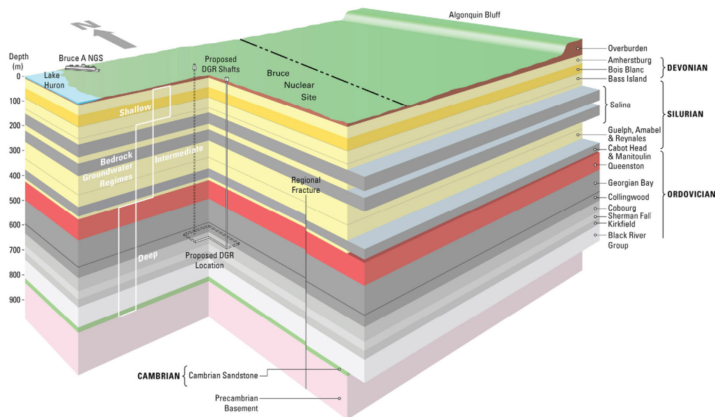
Figure 2: Illustration of Bruce site Descriptive Geosphere Model
