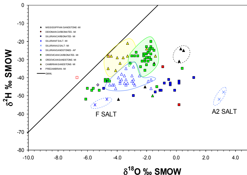
Figure 7: Southwestern Ontario Isotopic Signatures 2 H – 18 O for groundwaters with salinities > 100 g L -1 .
